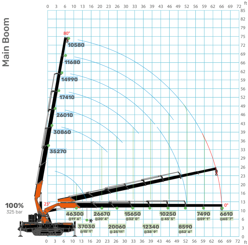
Hydraulic Jib
